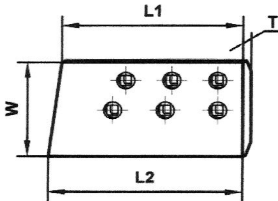
TYPE 1 (Finish)
